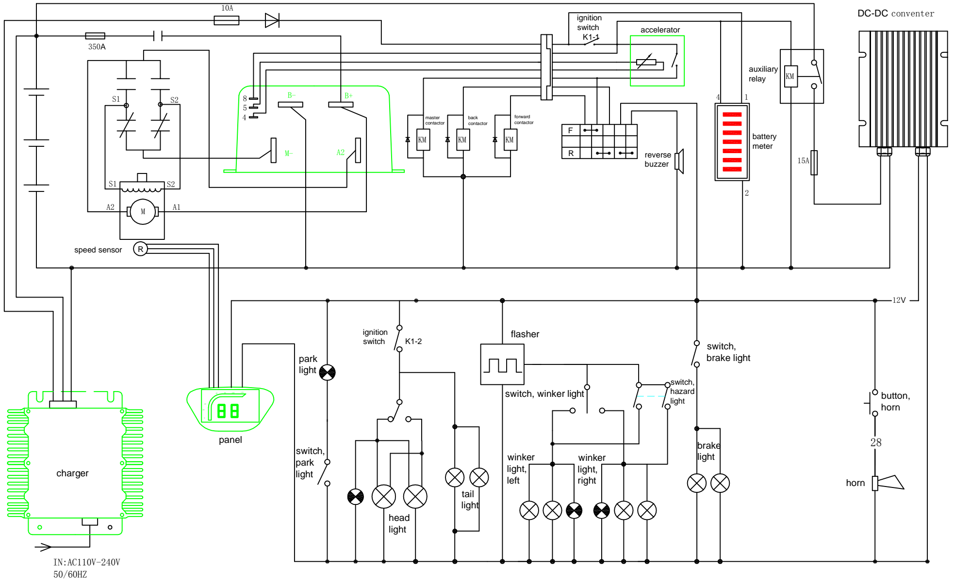
48V Electric Vehicle Wire Diagram
